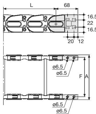
Fig. A End brackets can be mounted in any position. (Fig. A)
