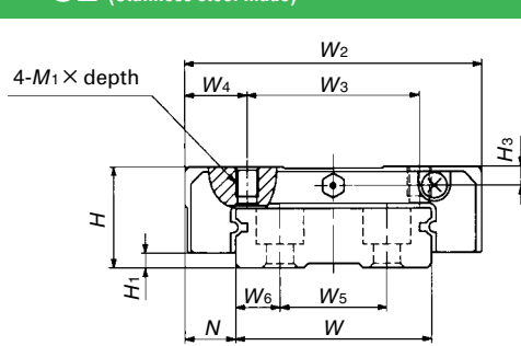
LWFS 33(...SL) LWFS 37(...SL)
