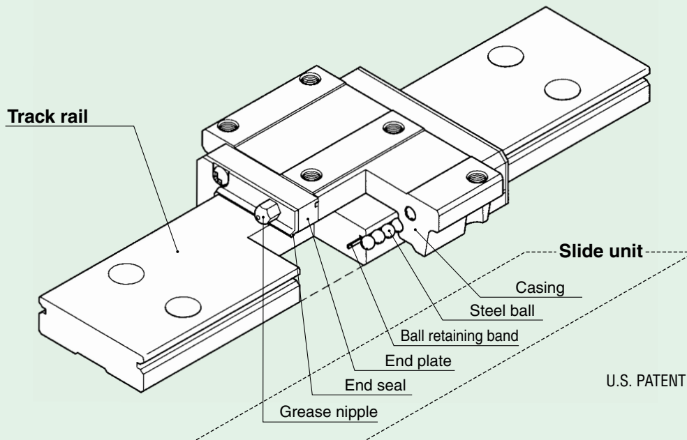
Structure of Linear Way F
