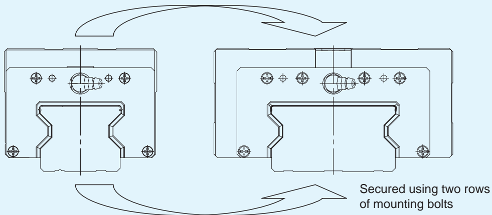
Fig. 3 Comparison between Models SRW and SRG in Cross Section
